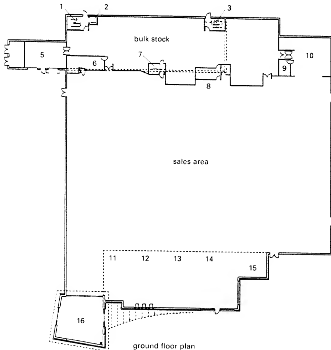
② Floor plan of a Sainsbury's supermarket in the UK (courtesy of Pick Everard)
